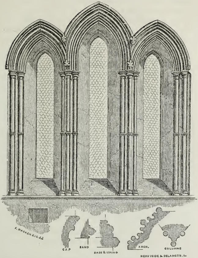
90. Polebrook, Northants, c. 1220.
